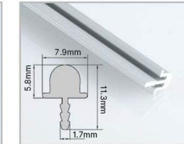
WSP-21 Sliding Bottom Profile
