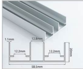
WSP-01 Sliding Top Profile
