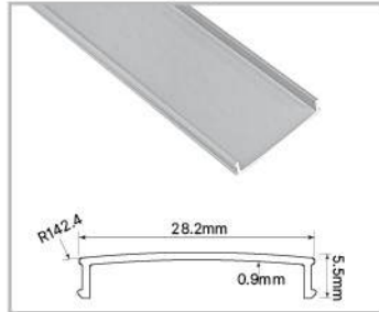
WSP-06 Sliding Top & Bottom Profile WSP-12C Bottom Cover Profile
