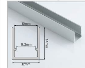
WSP-02 Sliding Top Profile
