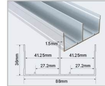
WSP-10 Sliding Top Profile
