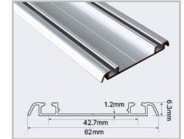
WSP-10 Sliding Bottom Profile
